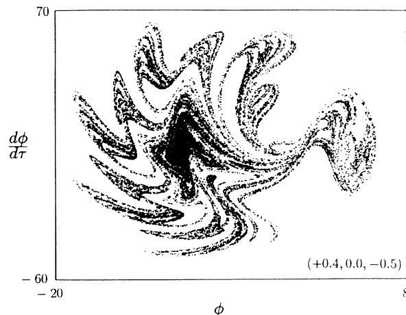
FIG. 6. Poincaré section of a chaotic solution found for the first excited state with \hbar v=0.085(\Phi_0^2/L_{eff}) , \hbar\omega_0=0.043(\Phi_0^2/L_{eff}) , \phi_{dc}=0.4 , K^2=0.3 , and i_{in}=0.18 .
