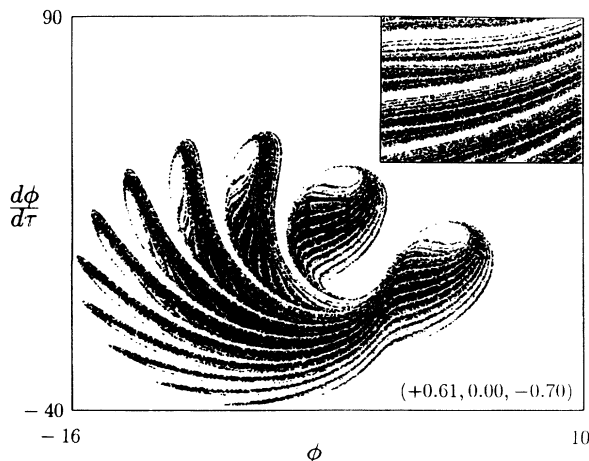
FIG. 5. Poincaré section of a chaotic solution found for the ground state with \hbar v=0.075(\Phi_0^2/L_{eff}) , \hbar\omega_0=0.043(\Phi_0^2/L_{eff}) , \phi_{dc}=0.5 , K^2=0.15 , and i_{in}=0.25 . The inset shows some of the fractal structure of the Poincaré section in more detail.
